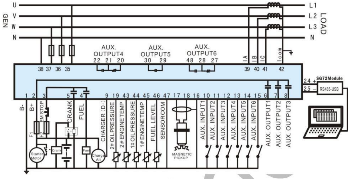
HGM8110A Typical wiring diagram
